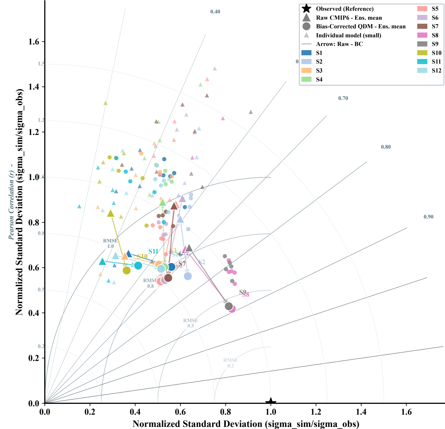
(a) Station Colours - Monthly Scale Each colour = one station | Large marker = ensemble mean
