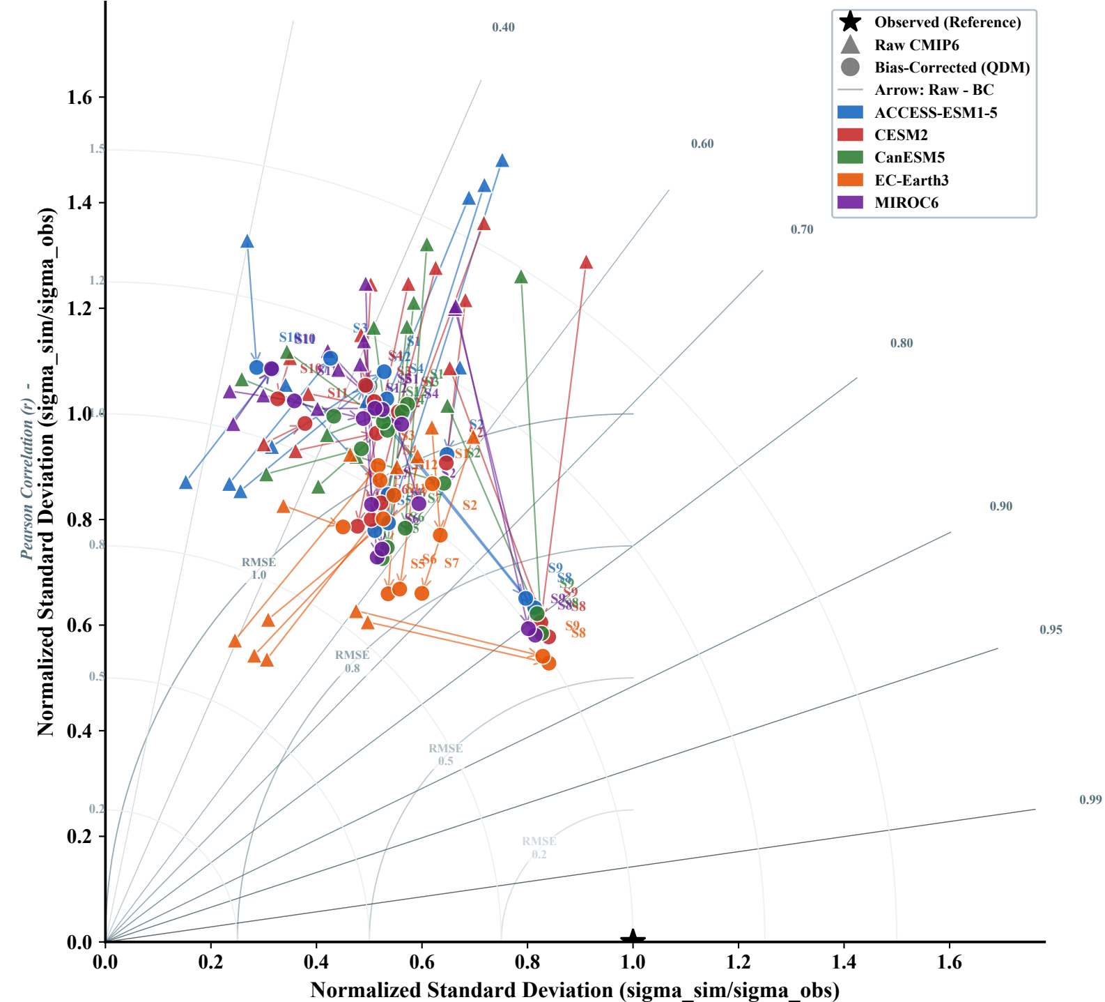
(b) Model Colours - Monthly Scale Each colour = one CMIP6 model | All stations shown
